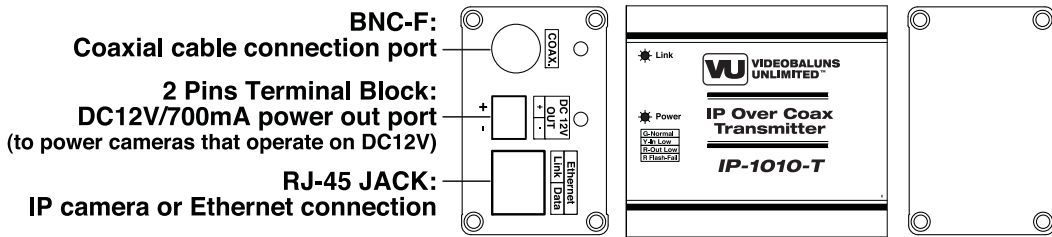
IP-1010-T , Transmitter
